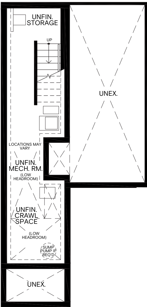
Basement
