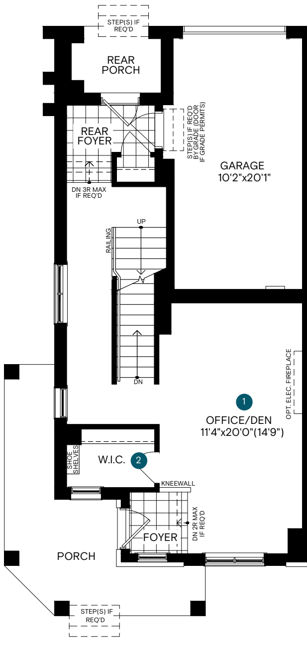
Ground Floor — Designer Choice Options
