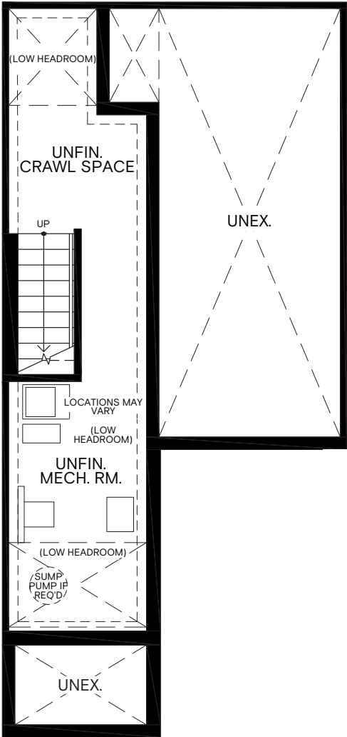
Basement
