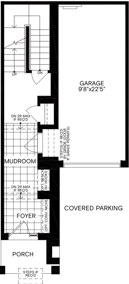
Second Floor — Designer Choice Options
