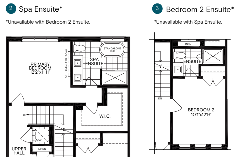
Second Floor – Designer Choice Options
