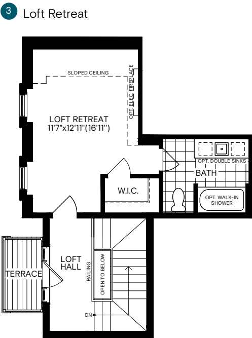
Loft - Designer Choice Options
