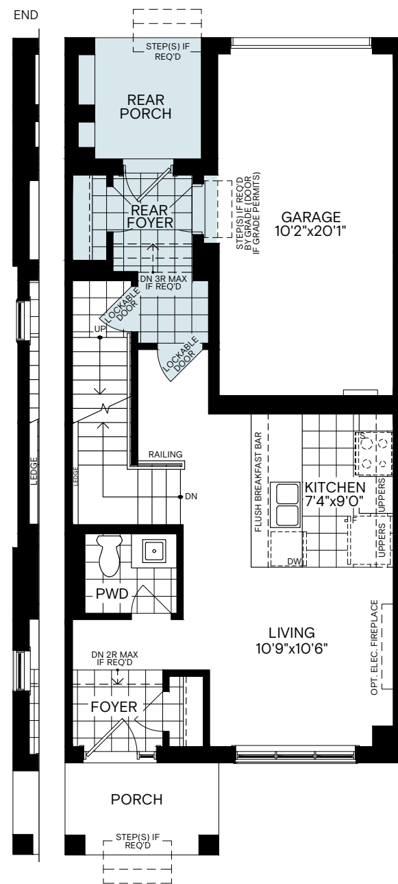
Ground Floor Lower Residence
